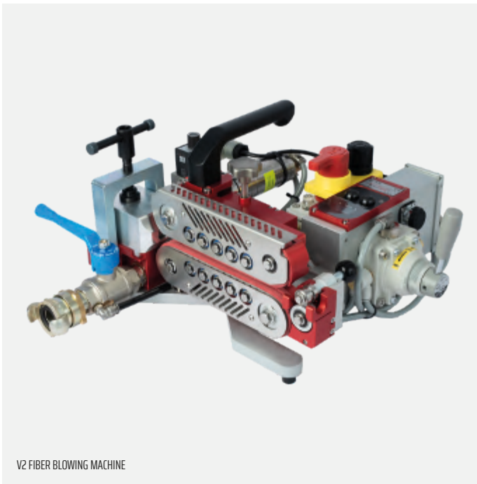
V2 FIBER BLOWING MACHINE
